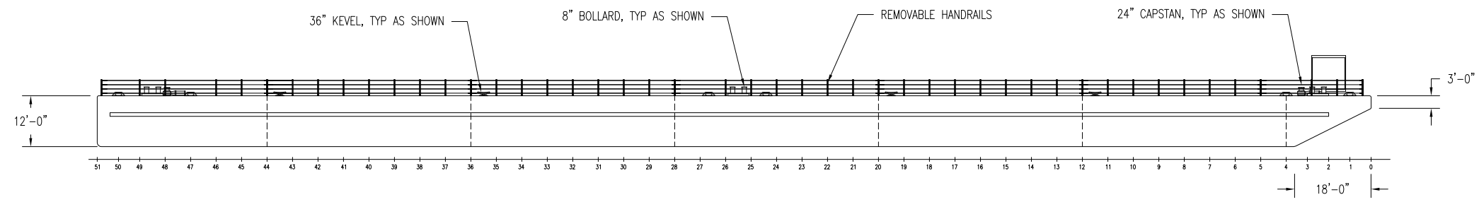
OUTBOARD PROFILE
